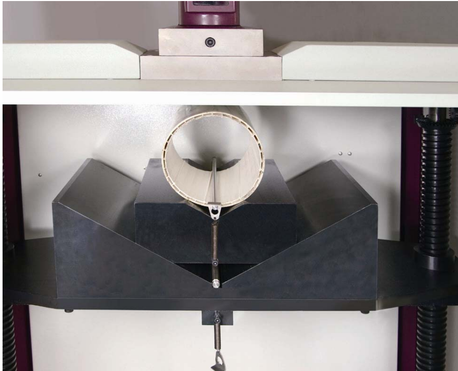
Medium vee-block
